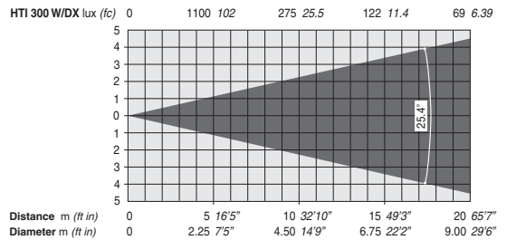
Lens 1:1.6/100 mm (25.4°) - with light frost
