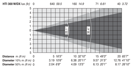
Lens 1:1.6/100 mm (23.1° - 35.4°) - with heavy frost
