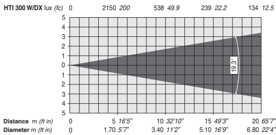
Lens 1:2.2/135 mm (19.3°) - Standard
