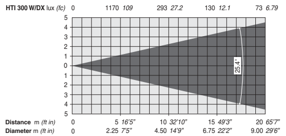
Lens 1:1.6/100 mm (25.4°) - Available on request
