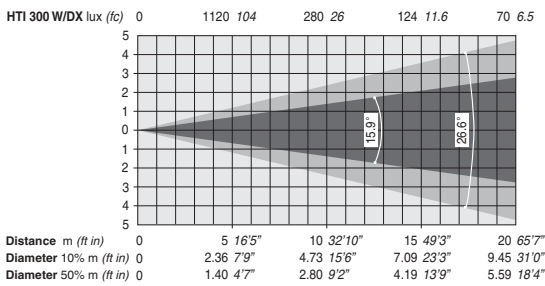
Lens 1:2.2/135 mm (15.9° - 26.6°) - with heavy frost
