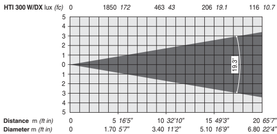
Lens 1:2.2/135 mm (19.3°) - with light frost
